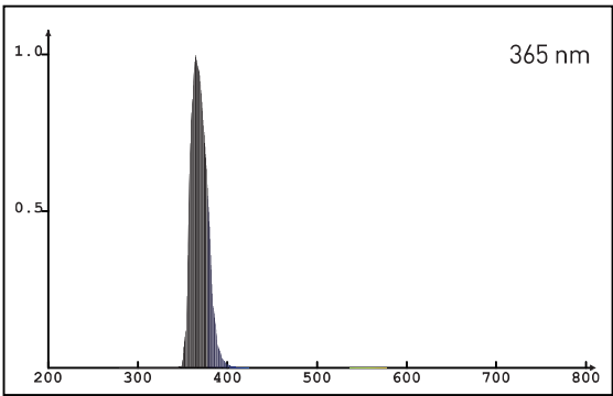
LED UVA Spectrum
